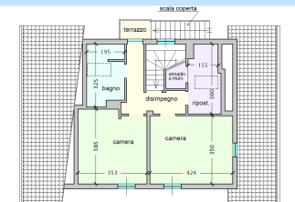
PIANO MANSARDATO
